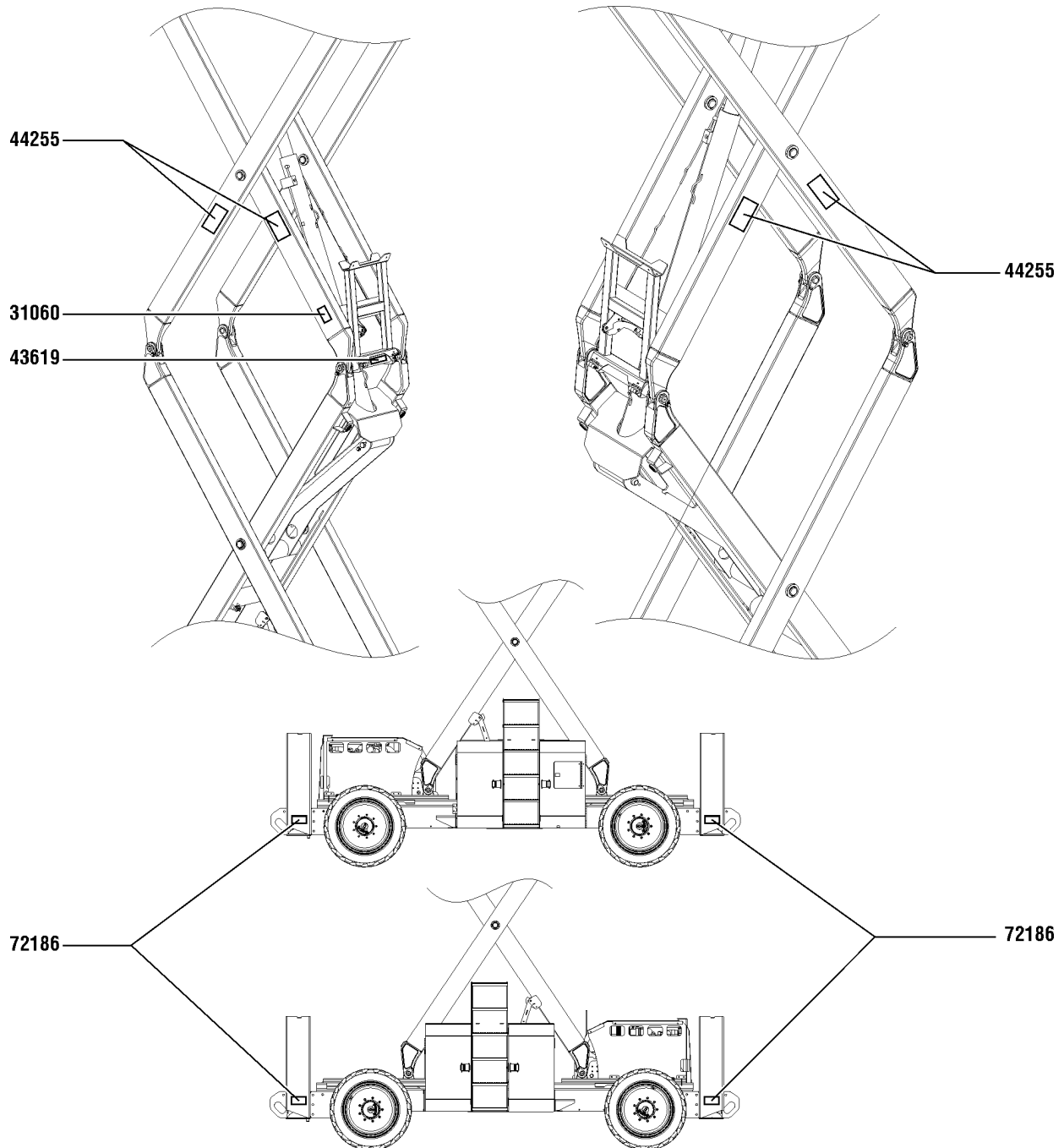
Ground Control Side
